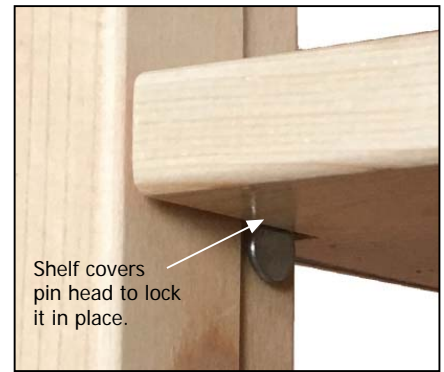
Recessed edge on our upright allows the head of the pin to be locked in place by the shelf.
